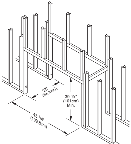
Figure 4 - Framing Firebox
