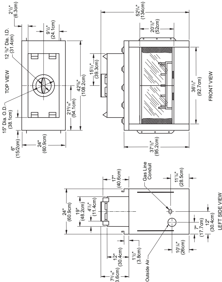
Figure 1 - (V)3612ST Dimensions
